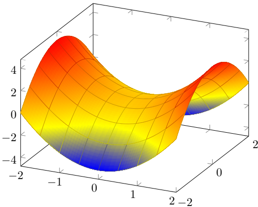
Figure 1. Hyperbolic paraboloid obtained from PGFPlots [PFGPlots].
